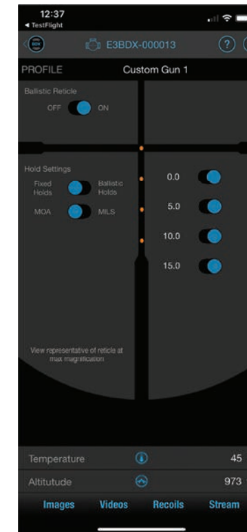
BDX Application
